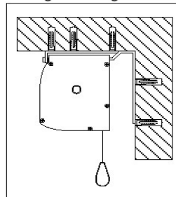
Ceiling Mounting
