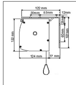
Cabinet dimensions
