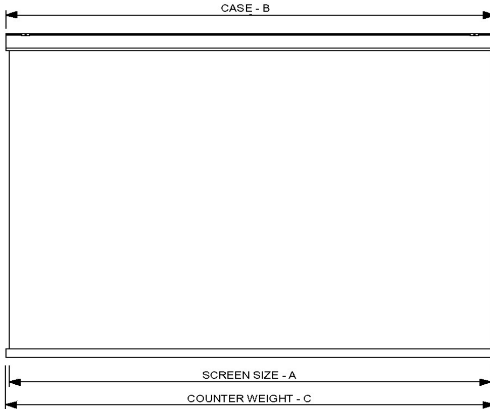
Concealing counterweight
